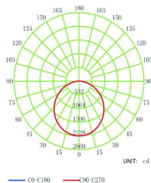
1X4 40W LED SURFACE MOUNT BACKLIT PANEL LUMINOUS INTENSITY DISTRIBUTION DIAGRAM
