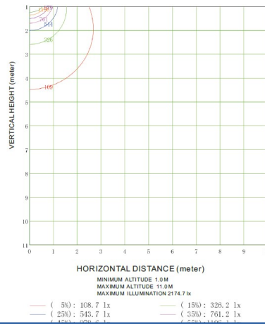
VERTICAL EQUILUMINOUS CURVE
