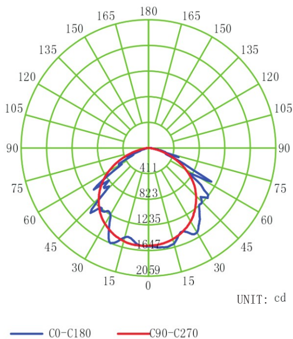
LUMINOUS INTENSITY DISTRIBUTION DIAGRAM
